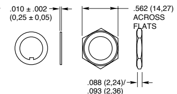
Keyed Washer
