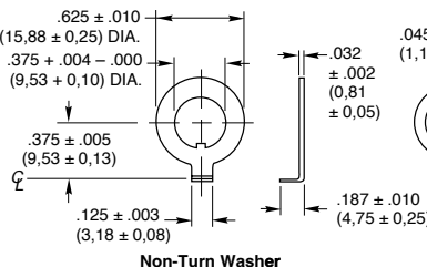
Non-Turn Washer
