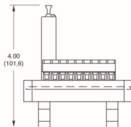
DIN-Rail Mount
